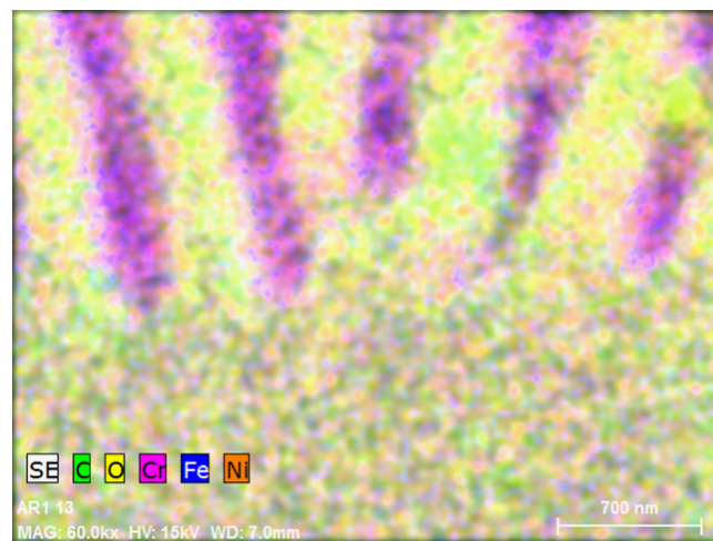
Fig. 3. A representative EDS X-ray map of \text{SS} \parallel NLL-treated surface (stripes produced by the treatment are located in the upper half of the image, whilst the untreated steel is visible in the lower half).
